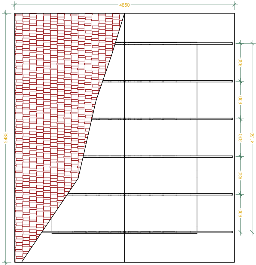
1 STR DENAH KUDA-KUDA 1:50
