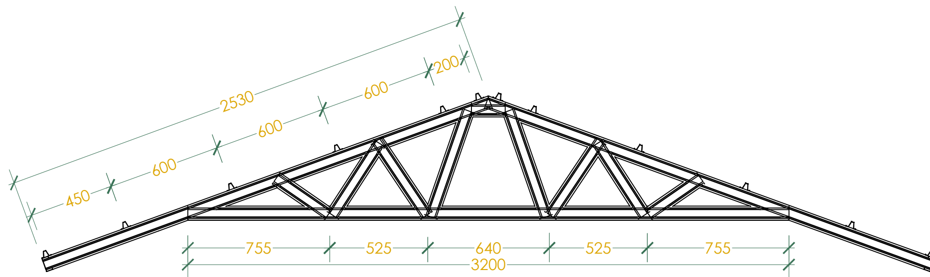
1 STR DETAIL KUDA-KUDA (6 BH) 1:20
