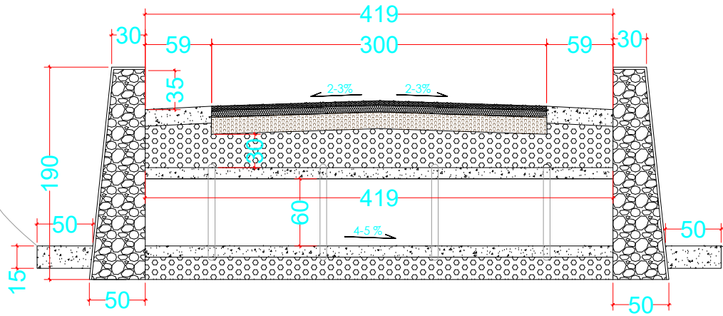
TIPYCAL GORONG-GORONG
